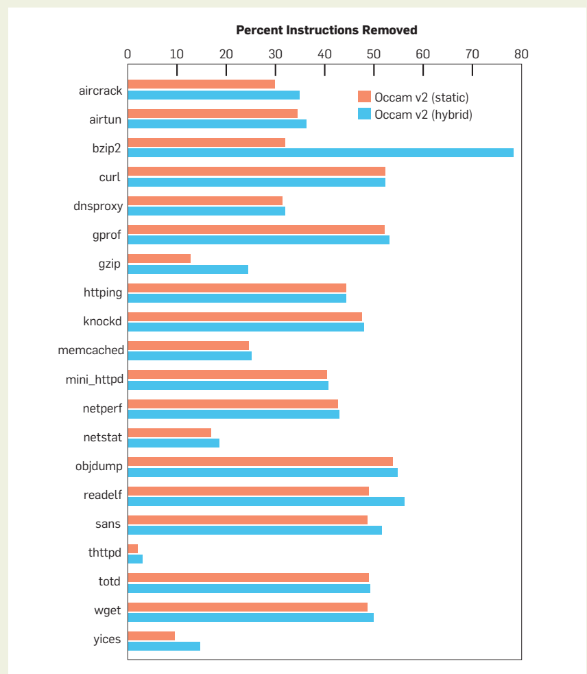
Figure 2. Percentage of instructions removed.
