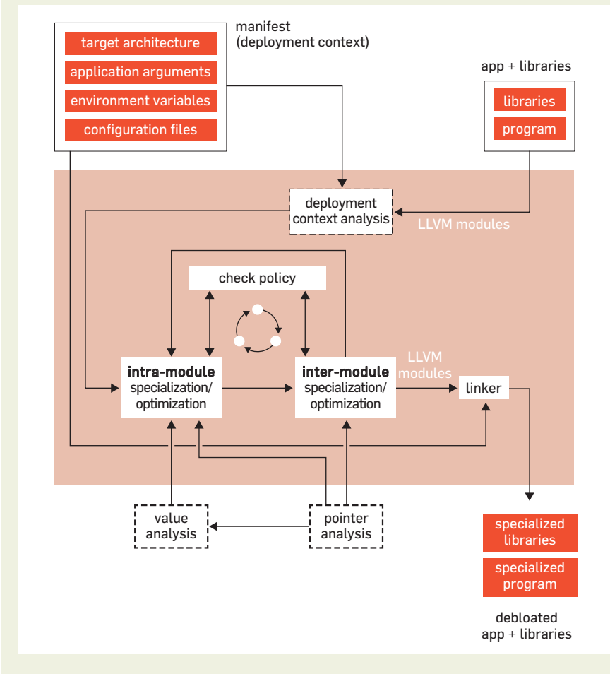
Figure 1. Overview of OCCAM's workflow.
